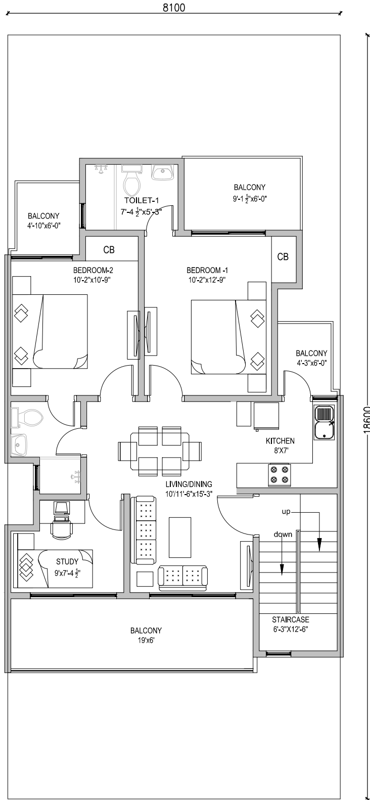
FIRST FLOOR PLAN SUPER AREA : 1093 SFT (101.54 SQM)
